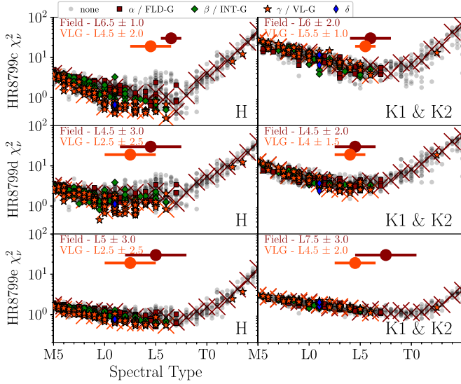
Figure 8. We plot \chi^2 between our GPI spectrum and each object in the spectral libraries described, as a function of spectral type of field objects for each planet. From top to bottom, we plot planets c, d, and e. The left shows the \chi^2 for the H band, the right shows the \chi^2 for the combined K1 and K2 bands. The large red and orange points at the top of each panel represent the mean and 1 - \sigma error for the best fit SED for field and VLG objects, respectively. We indicate gravity classification via the legend at the top. Spectral standards for FLD-G (Kirkpatrick et al. 2010; Burgasser 2014) and VL-G (Allers & Liu 2013) are indicated by red and yellow crosses, respectively.
